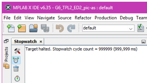
STOPWATCH RETARDO 1s
