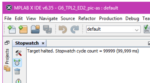
STOPWATCH RETARDO 100Ms
